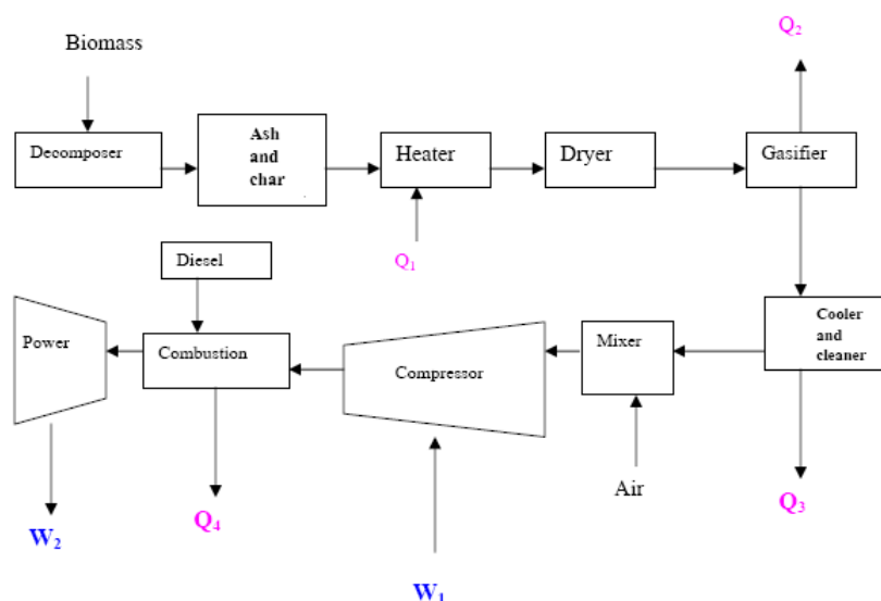
Figure 7. Advanced biomass power with diesel engine (Omer, 2006).
