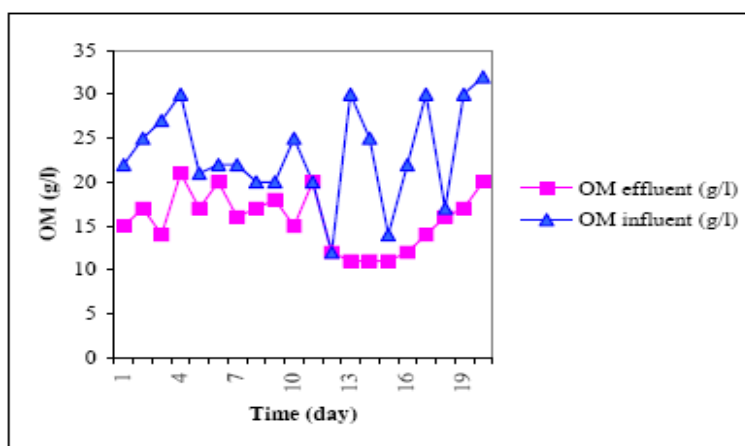
Figure 5. Organic matters before and after treatment in digester (Omer, 2006).
